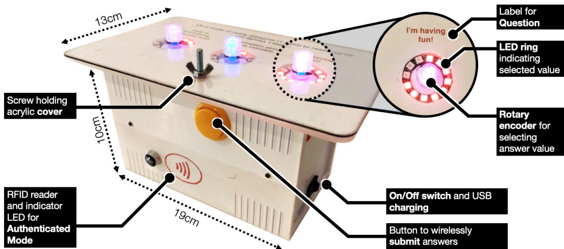
Figure 2. The EvalMe Sender is passed between students to collect answers from students to a 3-question questionnaire. Answer types can be categorical or numerical. LEDs indicate the selected response.
